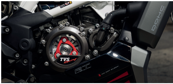
Reverse-inclined 310cc engine with race-tuned fuel injection.
